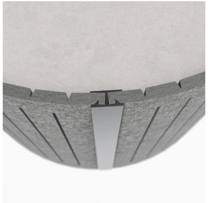
Zintra Taiko Aluminium Joiner Detail
